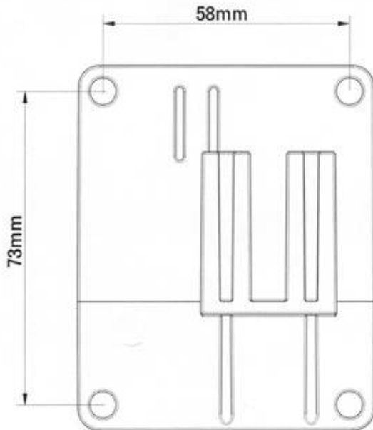
Figure 1 Bracket mounting holes: 4 holes, 5.5mm diameter
