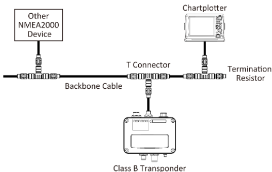
Figure 8 NMEA2000 Network
