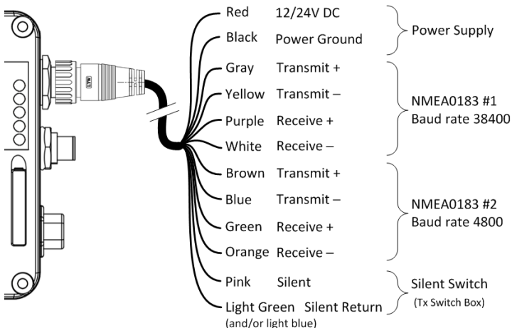
Figure 7 Wiring instructions
